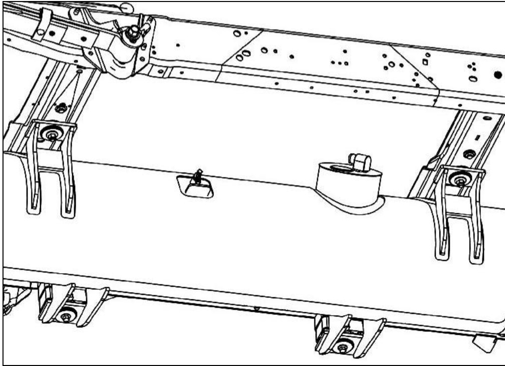
View of inboard cross member mounts (driveshaft removed for clarity).
