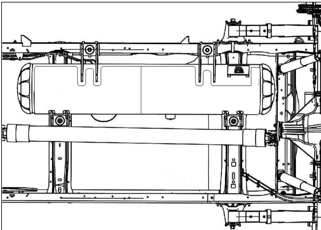
Bottom view illustrating a fully installed tank.
