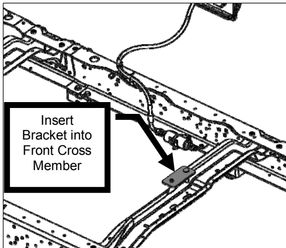
View looking from above frame.
