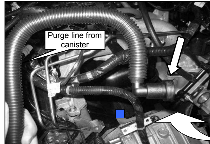
Before Rotation Rotate VMV hose 180 degrees to align with throttle body.
